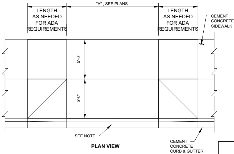
DRIVEWAY SEPARATION (MEASURED FROM BOTTOM OF THE TAPERS)
