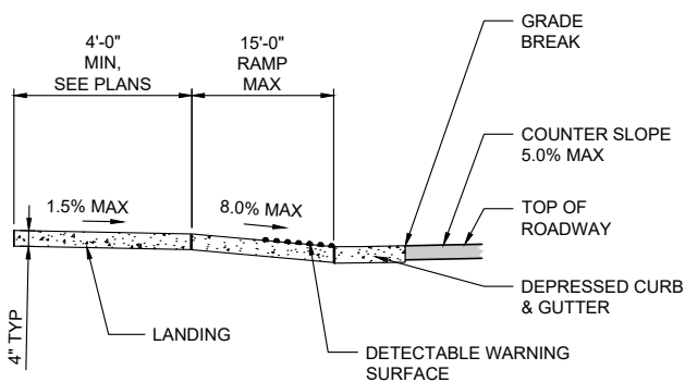
SECTION C NTS
