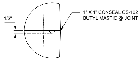
JOINT DETAIL A
